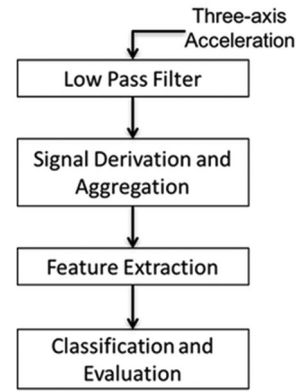
Fig. 3. Sleep stage extraction flowchart.
